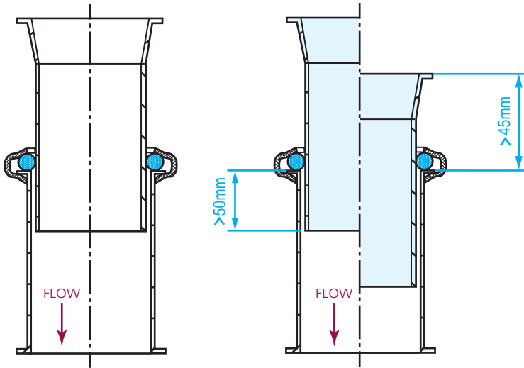
Connection of tubes 1 – 3mm wal thickness
